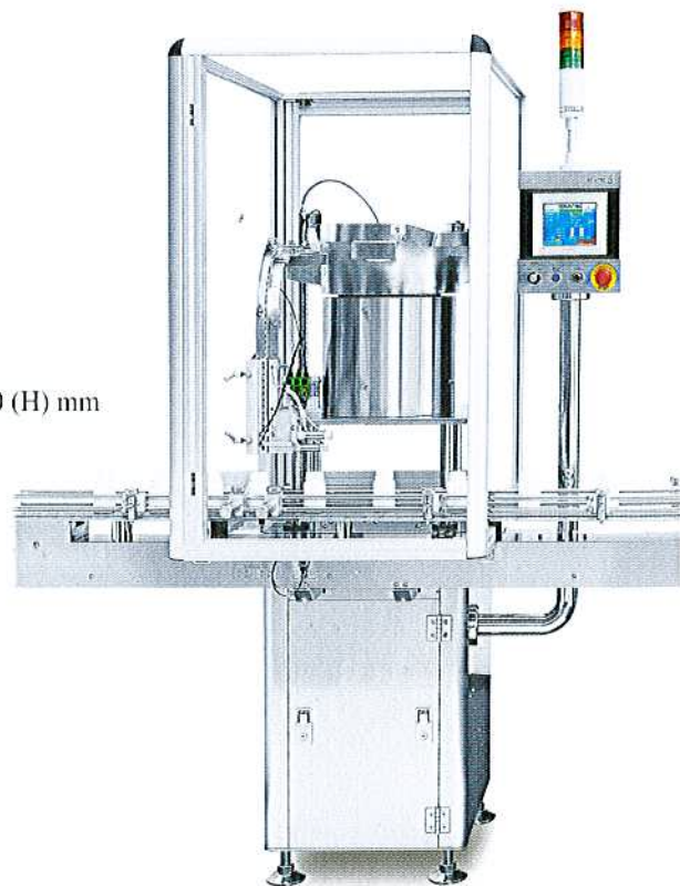
Fully interlocked guarding
