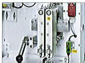
Automatic position alignment side gripping belts
