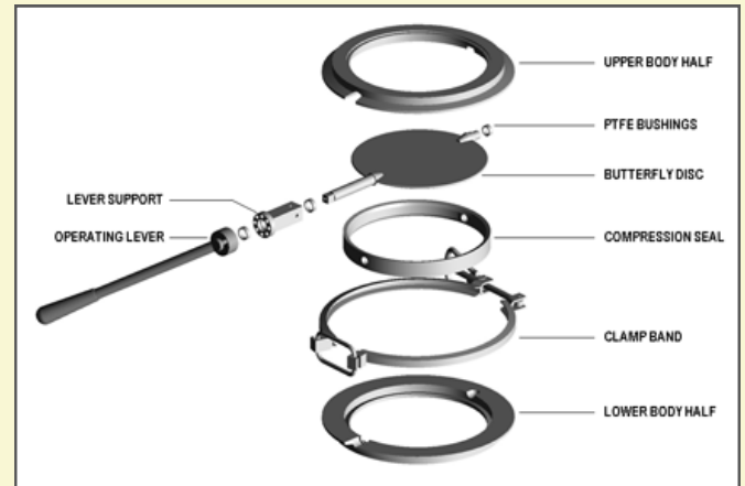
Exploded view of Model CV Valve with manual operating lever
