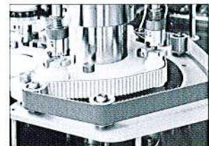
Bottle clamping timing belt
