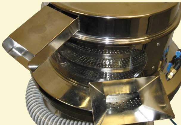
Continuous TIG Welded Spiral Dedusting Tray
